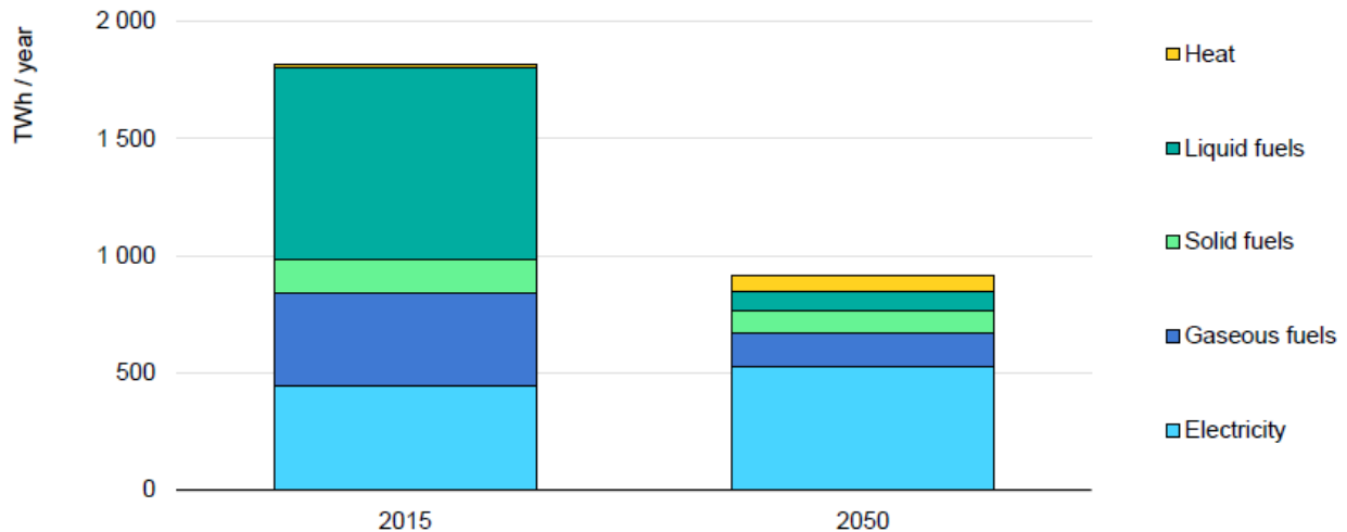
Figure 2.2 Final energy consumption by energy vector, 2015 and 2050
